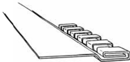
Double Fold Offset Seam
